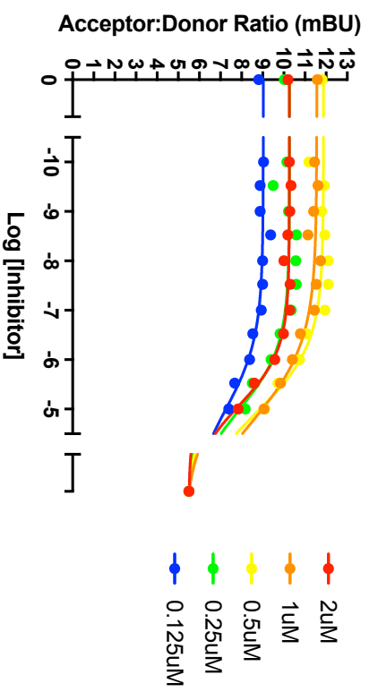
CDK13-NL-K Tracer 7281 AT-7519
