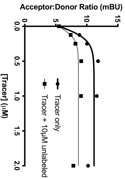
CDK13-NL-K Tracer 7281 AT-7519 EC50
